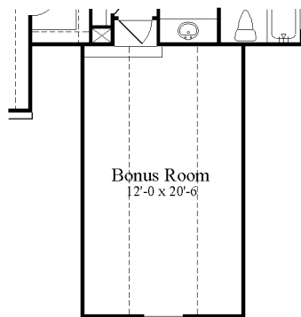
Opt. Bonus Room
